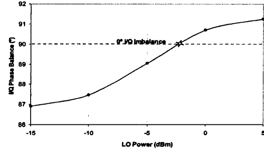
Fig. 6. Simulated phase balance between the IF outputs of the I and Q mixers at f_{RF} = 5.15 GHz and f_{LO} = 2.57 GHz. The desired phase difference of 90^\circ is noted.
