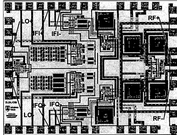
Fig. 8. Layout of direct-conversion receiver currently in fabrication. Chip area is \sim 2.3 mm x 1.8 mm.
